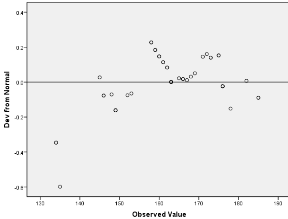
Detrended Normal Q-Q Plot of KEPUASAN KERJA
