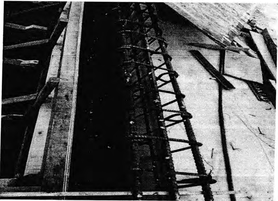
Gambar 3.5.7 Bekisting balok
