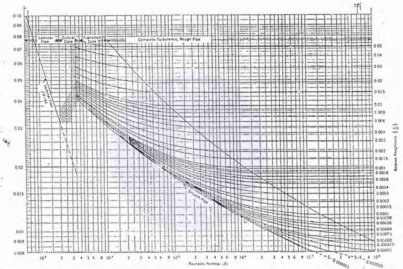
Fig. 16-2K. Moody Diagram for friction in pipe. The values for friction factor are on the vertical scale at left. (See Friction Manual © Hydraulic Institute.)
