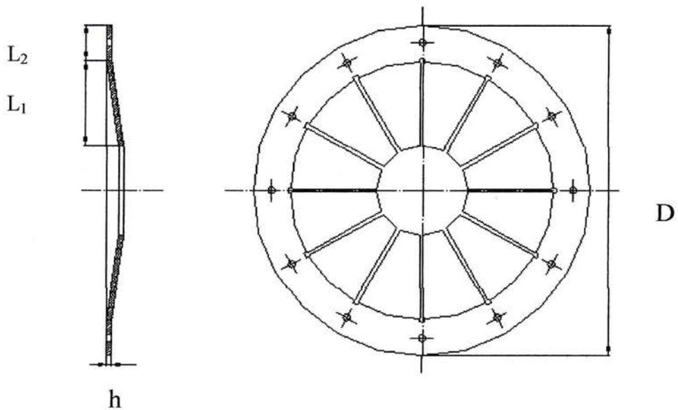
Gambar 8. 1. Pegas Matahari
