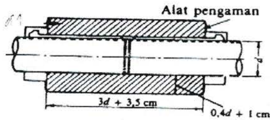
Gambar 2.1. Kopling Bus
