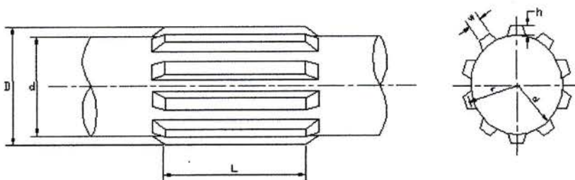
Gambar 4.1. Spline
