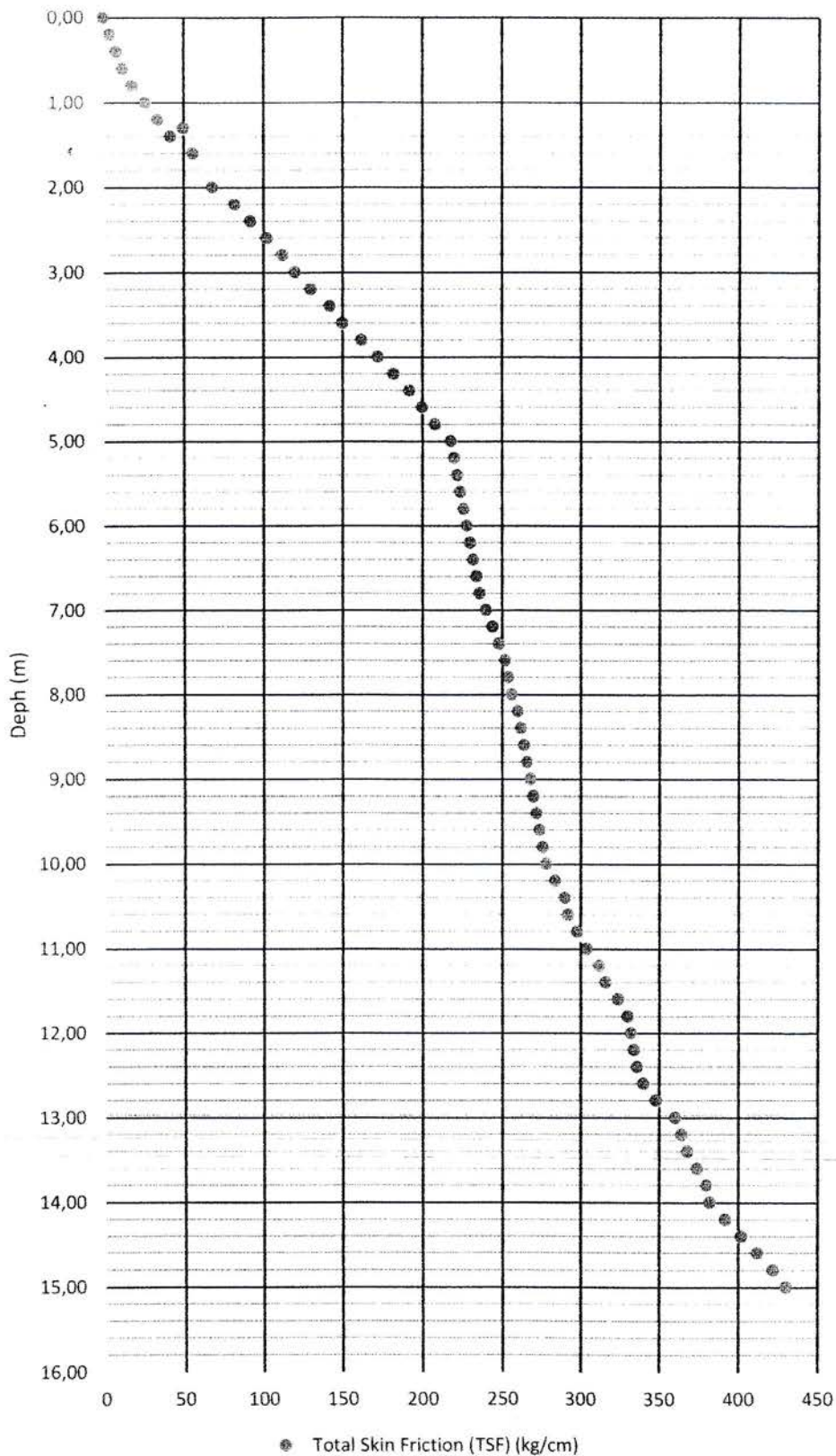
Graphic Sondring Total Skin Friction (TSF) (kg/cm)
