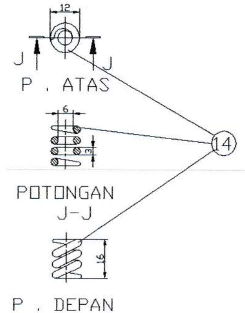
Gambar 3.5 Pegas
