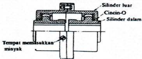
Gambar 2.8 Kopling Gigi
