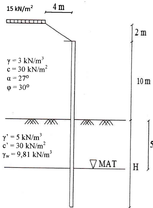
Gambar 4.3 Tampak Soldier Pile
