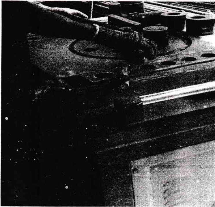
Gambar 3. 7 Bar Bending
